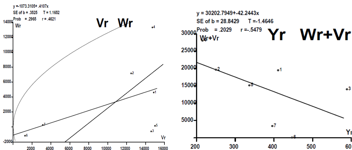
Fig.1. Coefficient of correlation ( r ) between the parental order of dominance ( Wr+Vr ) and parental measurements ( Yr ) i.e. r(Wr+Vr, Yr) for different traits in chilli
