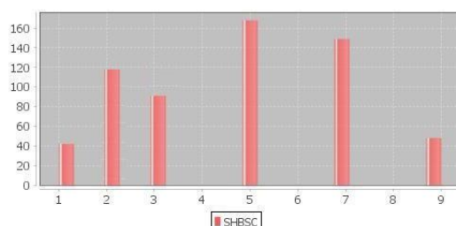
Fig. 1. Frequency distribution of SHB scores of RILs involving populations of Jasmine 85
