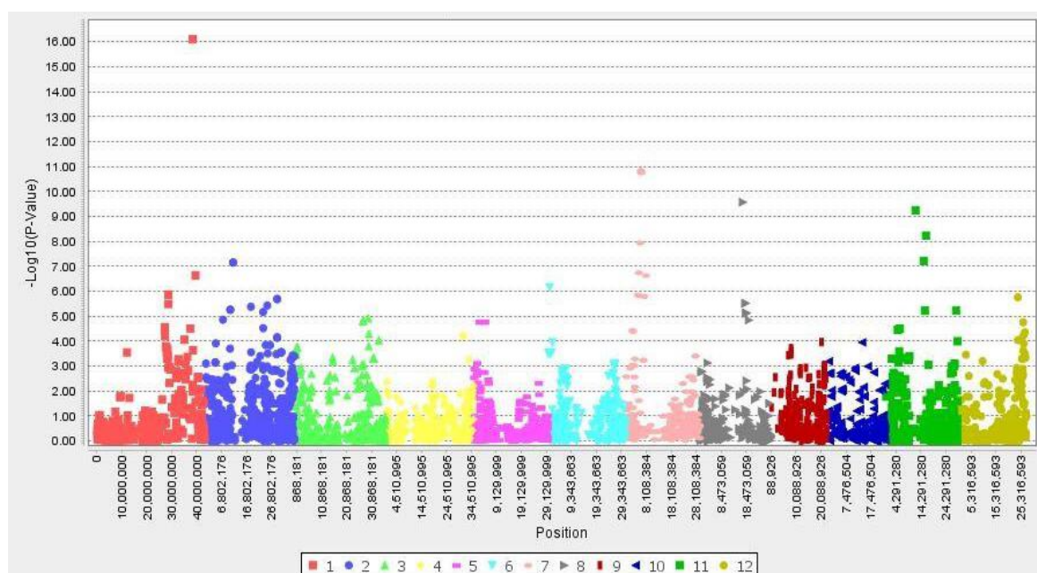
Fig. 5. Manhattan plot depicting genome-wide association results for sheath blight trait of Tetep populations using mixed linear model (MLM) for analysis
