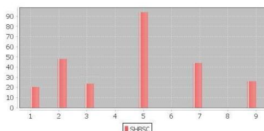
Fig. 3. Frequency distribution of ShB scores of RILs involving populations of MTU 9992
