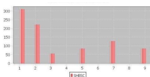
Fig. 2. Frequency distribution of ShB scores of RILs involving populations of Tetep
