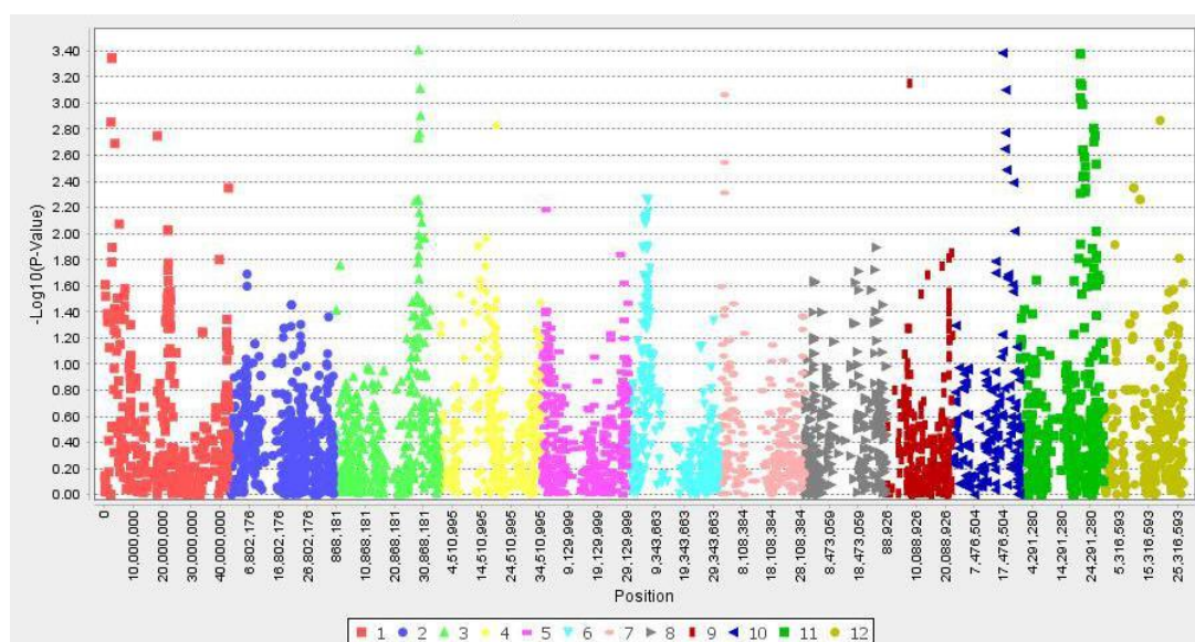
Fig. 4. Manhattan plot depicting genome-wide association results for sheath blight in Jasmine 85 populations using mixed linear model (MLM) for analysis
