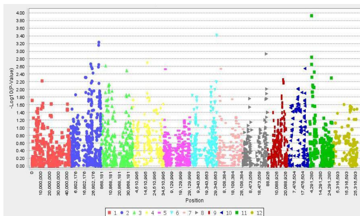
Fig. 6. Manhattan plot depicting genome wide association results for sheath blight trait of MTU 9992 populations using mixed linear model (MLM) for analysis
