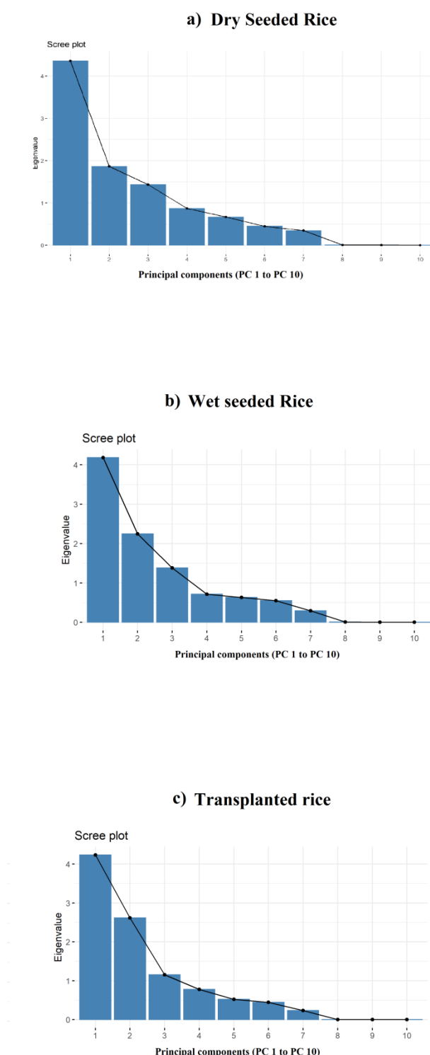
Fig. 1. Eigen values and its contribution over three different rice establishments
