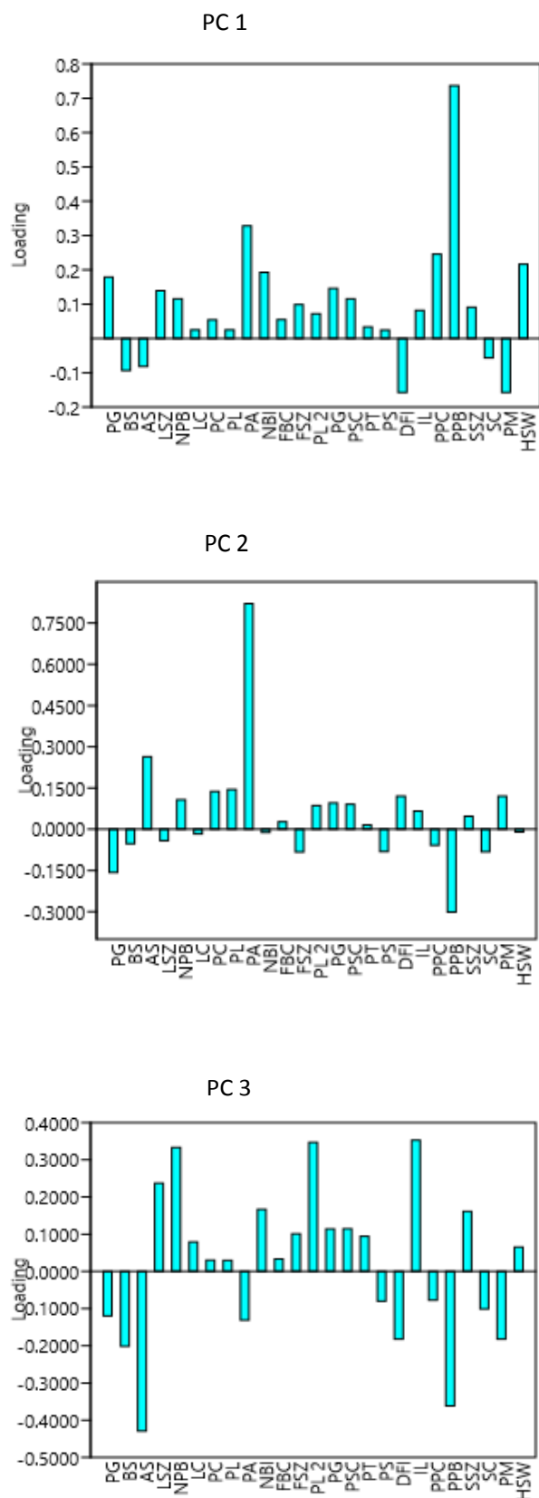
Fig. 1. Graphical representation of rotated component matrix for different traits in PC 1, PC2 and PC3
