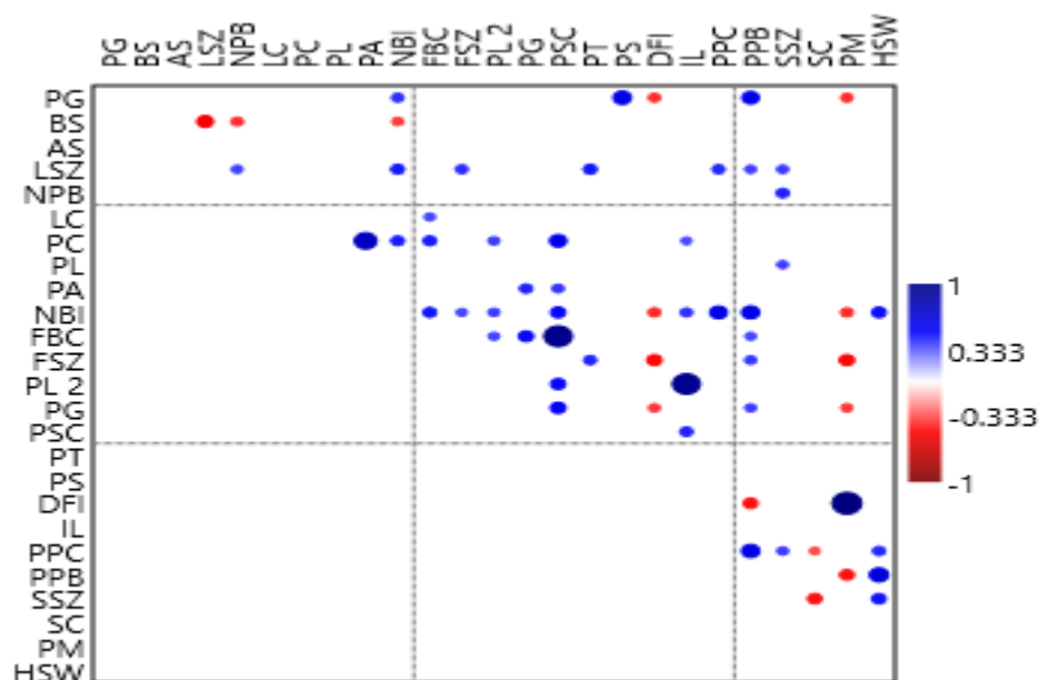
Fig. 4. Plot diagram of Correlation between different traits
